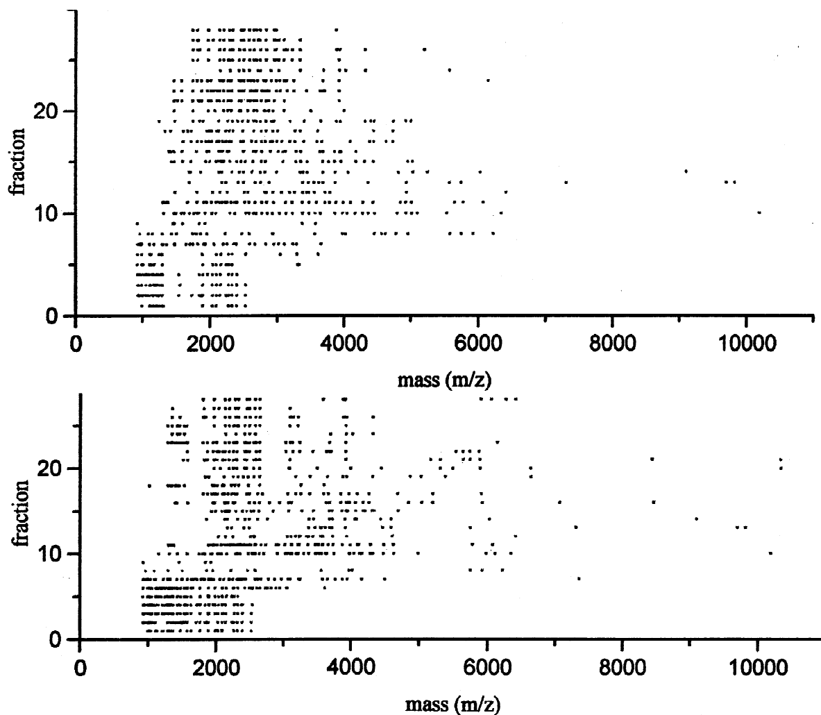
Fig. 2. Peptide maps from pH pool 1 (A) and pH pool 7 (B). The 2D maps were generated from MALDI–TOF–MS spectra of pH pool RP-fractions and contain the molecular mass in the x-dimension and the fractions in the y-dimension. Each asterisk represents a molecular mass. The masses with a spectrum intensity >500 are shown resulting in approximately 1500 masses per map. Without restriction of the spectrum intensity each map contains approximately 3500 masses. Maps demonstrate repeated detection of the same masses especially in the first and last fractions of each chromatography.
