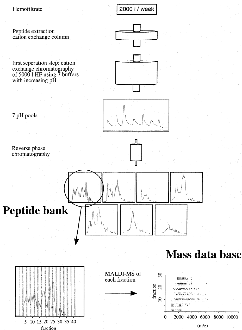
Fig. 1. Production of a human peptide bank and mass database from hemofiltrate. 2000 l hemofiltrate was collected per week. Extraction of the peptides was performed using a strong cation exchanger. Subsequently extracts of 5000 l HF were pooled and loaded on a 10-l cation-exchange column. Bound peptides were eluted using seven buffers with increasing pH. Each of the seven pH pools was rechromatographed on a reversed-phase column. Lyophilized aliquots of the fractions were analyzed on a MALDI-TOF-MS system. The MALDI-MS data of the fractions of each chromatography were accumulated in a one two-dimensional (2D) peptide map with the m/z values in the x-dimension and the fractions in the y-dimension. For each reversed-phase chromatography one 2D peptide map is produced.
